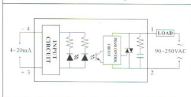
Connection Diagram
